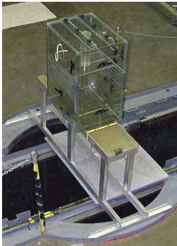
Figure 6. A high-angle view of the acrylic plastic NHP-restraint box centered on the table in the AFRRI ^{60}\text{Co} whole-body irradiator. The restrainer is secured to the table during animal irradiation with elastic straps. The table is immobilized by aluminum beams, secured to the bottom of the table, that contact the arcs located on the top of the pool. A water-filled PMMA cylinder used for dosimetry is located between the white ropes used for carrying the restraint box.
