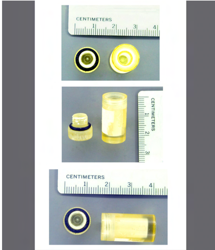
Figure 4. Vials for alanine pellets used at NIST and AFRRRI for irradiations under electron equilibrium conditions. (Photos provided by T.B. Elliott, PhD, and M.O. Shoemaker, PhD.)
